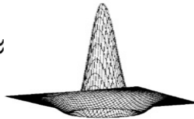
Laplacian
